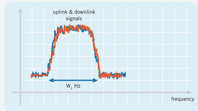
Channels overlapped by VPCMA-L to increase bandwidth capacity and cut bandwidth needs
