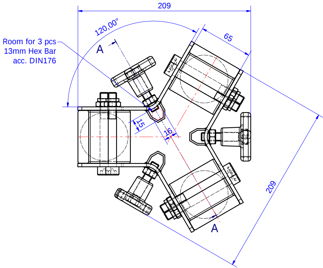
Illustration: Tripod leg
