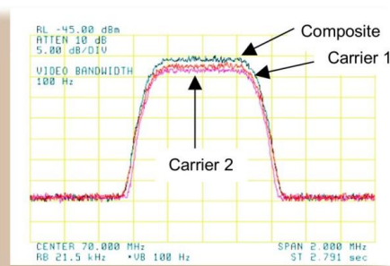
Figure 2: Duplex Link with DoubleTalk Carrier-in-Carrier
